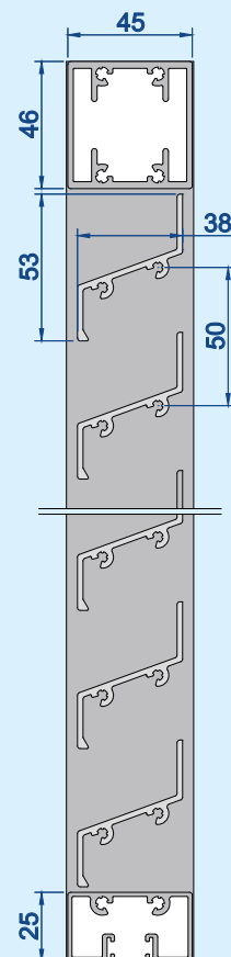
Vertical view: Scale 1:3
