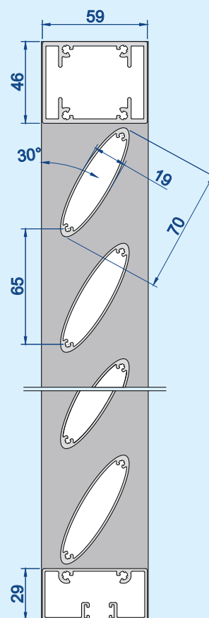
Vertical view: Scale 1:3
